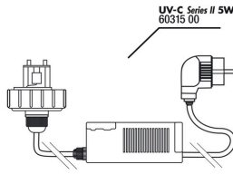
JBL AC UV-C 5 W ballast
