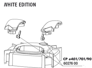
Stop cock set for JBL CP e4/7/9/15/1901/2
