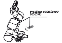
JBL PS a300/400 air connection
