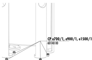
JBL CP e pump head grip
