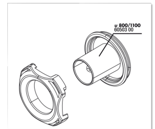
JBL PF "u" cover + hose connection
