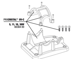
JBL PC UV-C 5,11,18,36 W mounting
