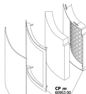
JBL CP m greenline Fixation FilterPad
